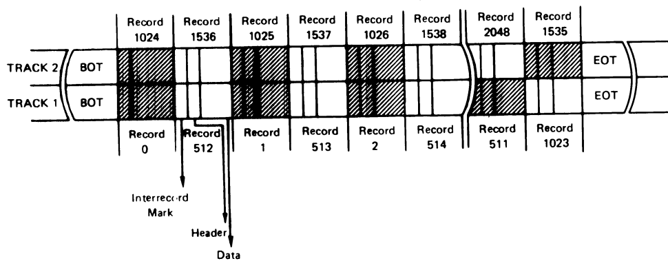
Figure 10–5: DECTape II Tape Format
