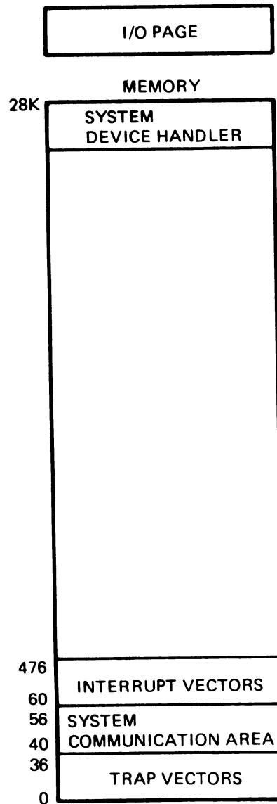
Figure 2-6: System Device Handler
