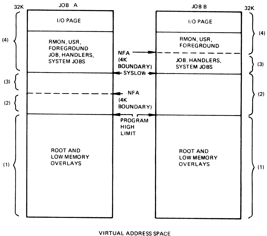
Figure 4-38: Background .SETTOP Summary
