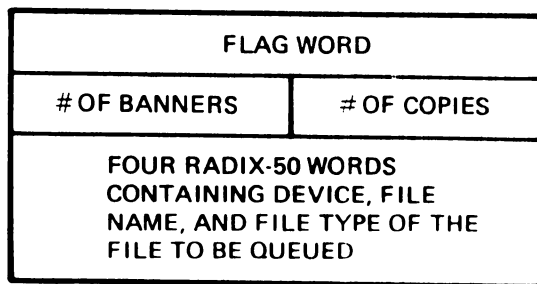
Figure 3-20: File Block
