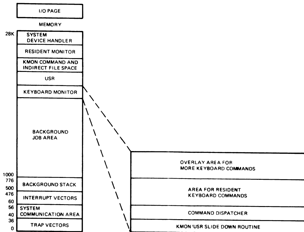
Figure 2-19: Keyboard Monitor
