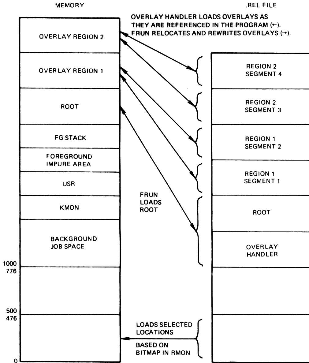
Figure 2-15: FRUN Command
