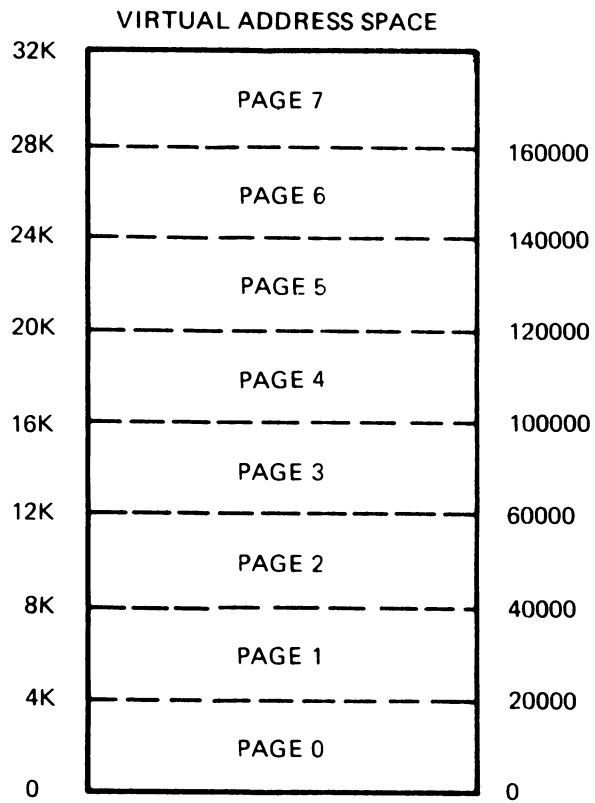
Figure 4-10: Smaller Pages
