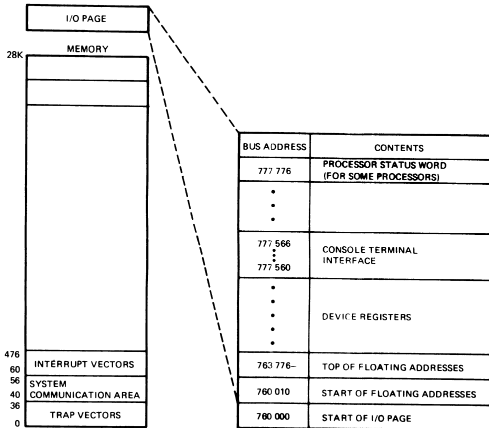
Figure 2-5: I/O Page
