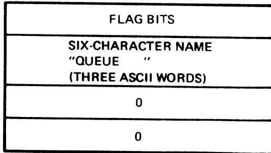
Figure 3-22: Request Acknowledgment Block
