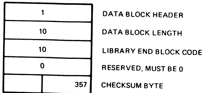
Figure 8–38: Library End Block Format
