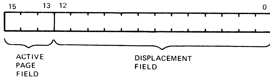
Figure 4-17: Virtual Address
