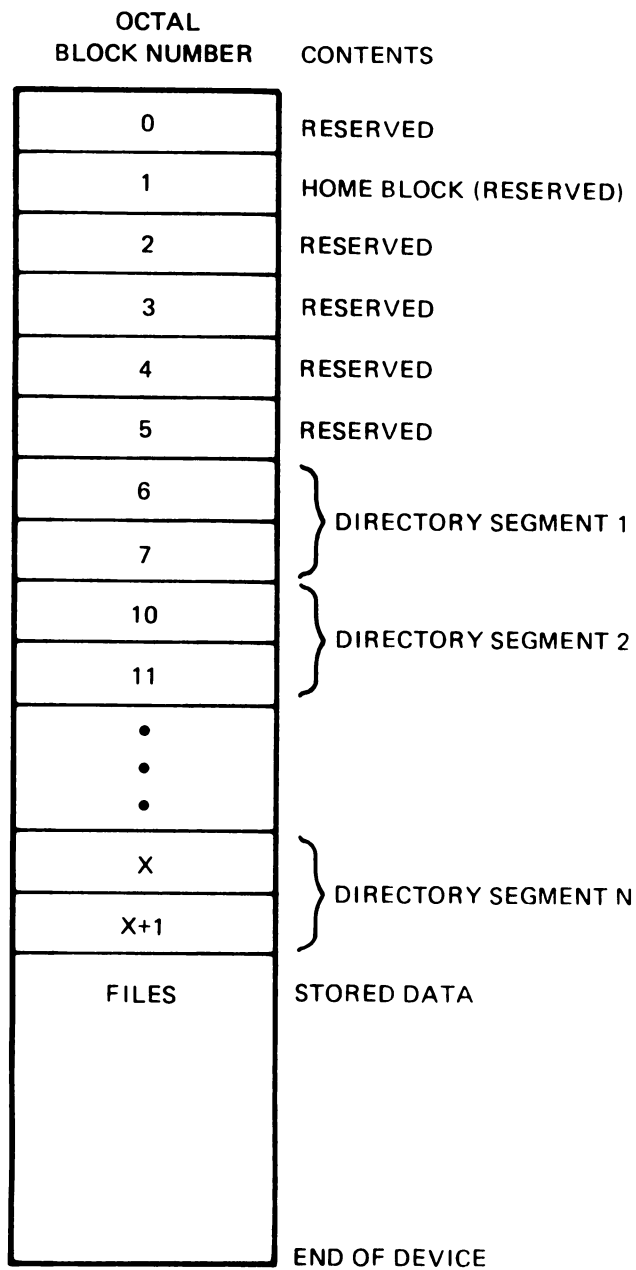
Figure 9-1: Random-Access Device
