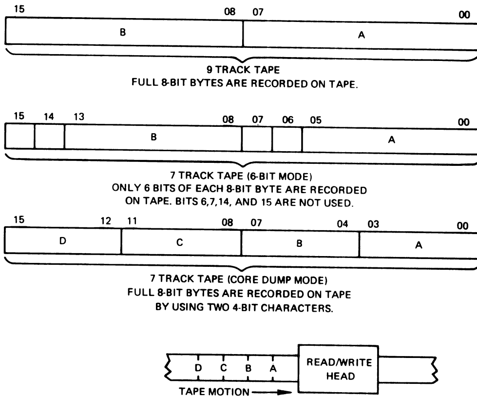
Figure 10-3: Seven-Track Tape
