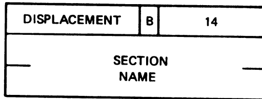
Figure 8–27: P-sect Displaced Relocation (Entry Type 14)
