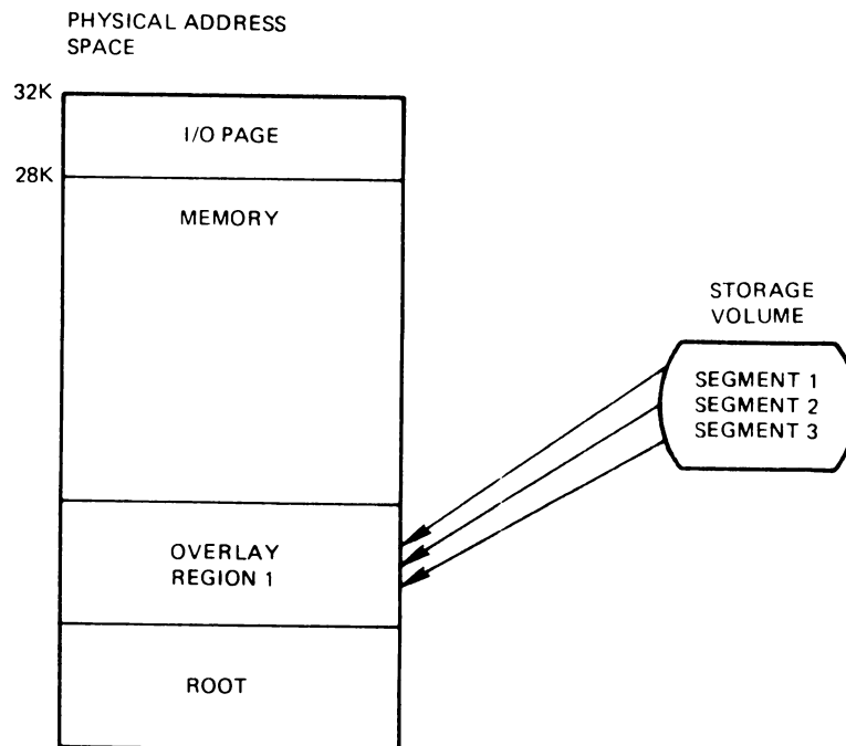
Figure 4-4: Overlaying
