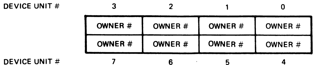
Figure 3-30: $OWNER Entry
