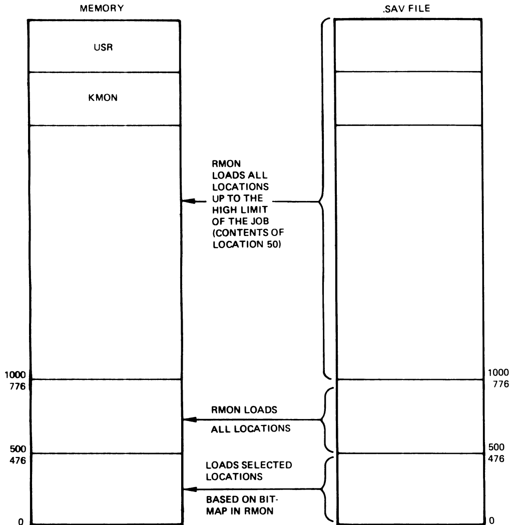
Figure 2-10: R Command
