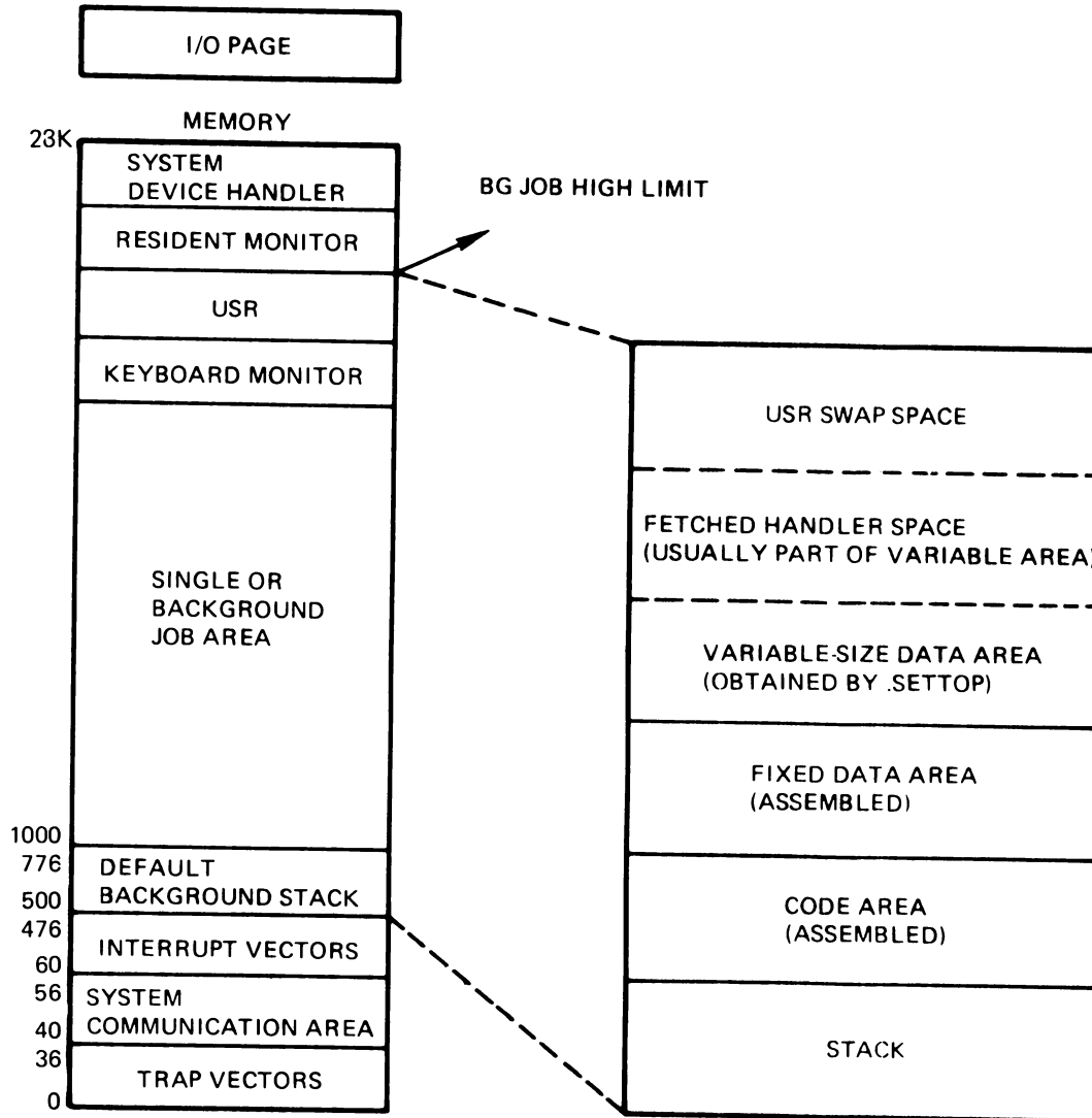
Figure 2-8: Background Job
