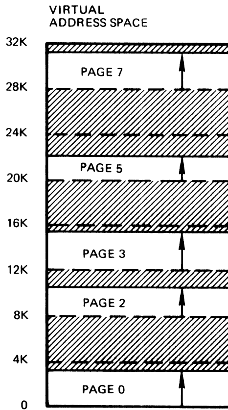
Figure 4-10: Smaller Pages
