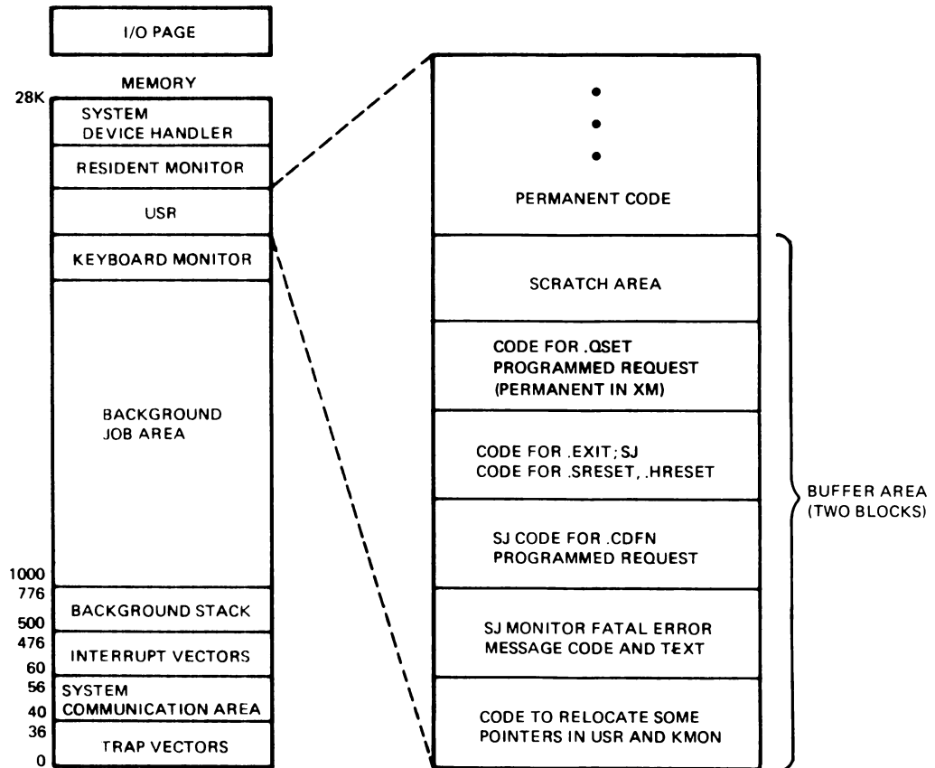
Figure 2-17: USR
