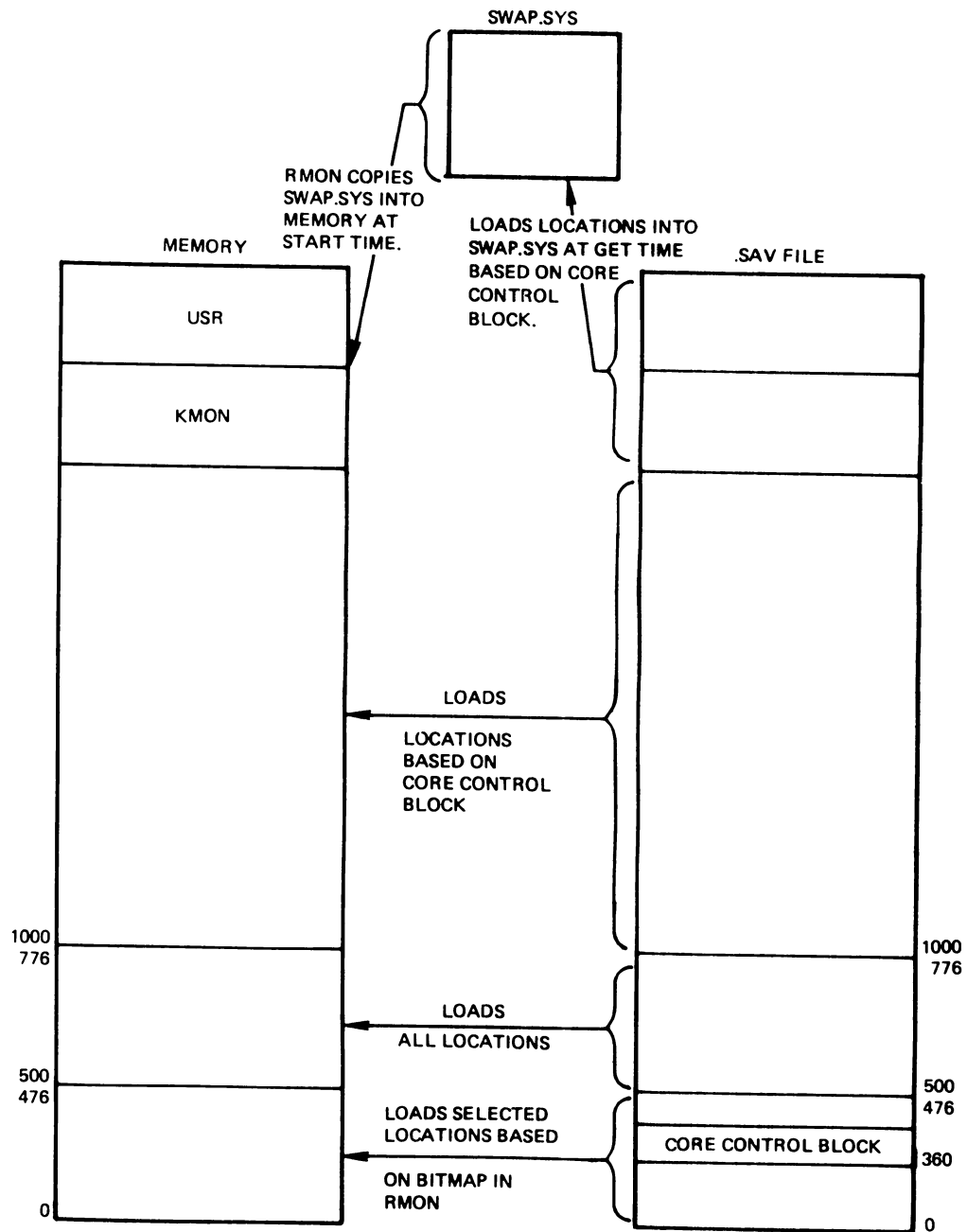
Figure 2-9: RUN Command
