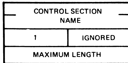
Figure 8–7: Control Section Name Entry Format (Entry Type 1)
