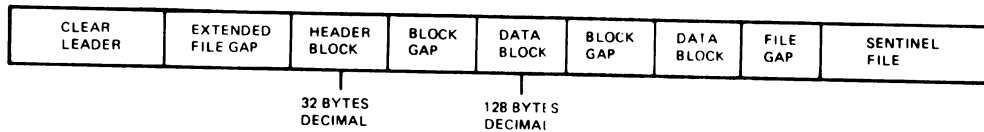
Figure 9-21: Cassette with Data
