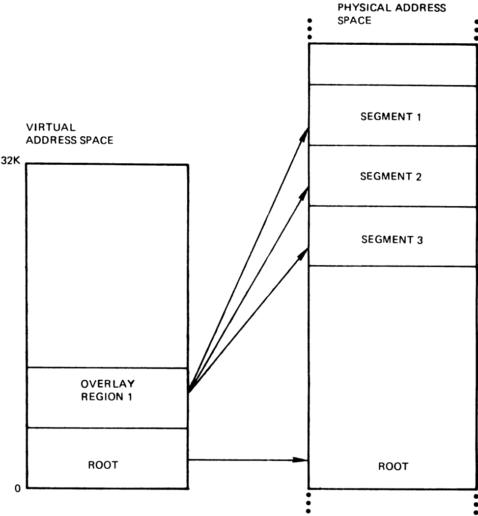
SEGMENTS 1, 2, AND 3 HAVE UNIQUE PHYSICAL ADDRESSES, BUT THEY TAKE TURNS USING THE SAME SET OF VIRTUAL ADDRESSES.
