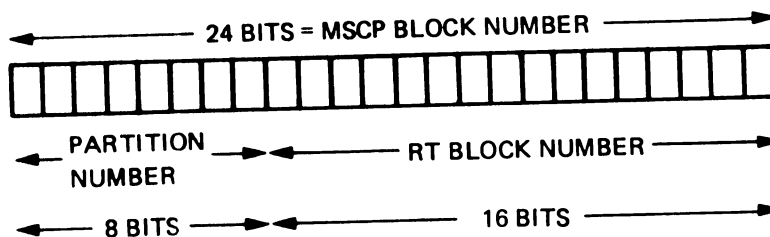
Figure 10-7: MSCP Disk Block Number
