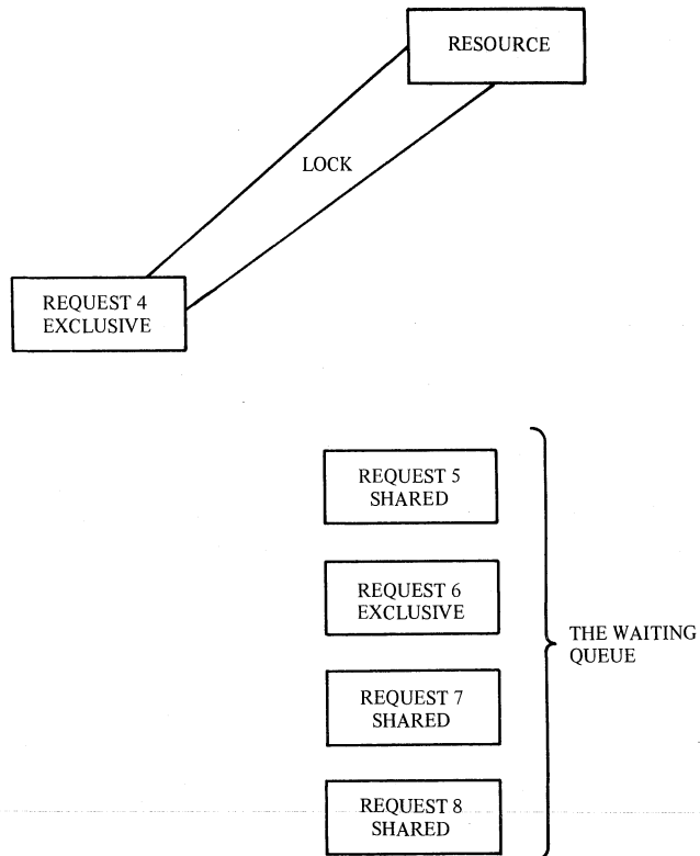
Figure 16-3. Exclusive Ownership
