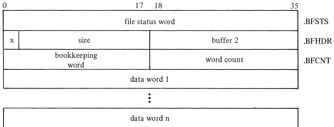
Figure 7-2. Buffer Structure
