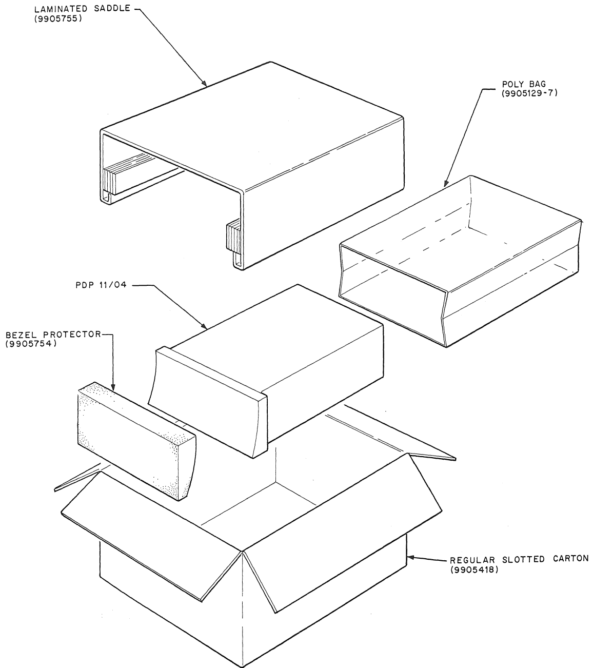
Figure 5-4 Packaging of PDP-11/04 [13.3-cm (5-1/4-inch Box)]
