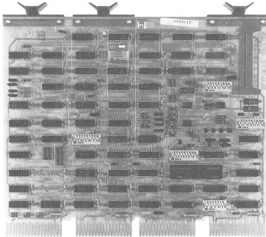
Figure 4-9 DL11-W (M7856) Switch Locations
