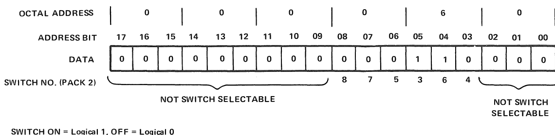
Figure 4-11 DL11-W Vector Address Selection
