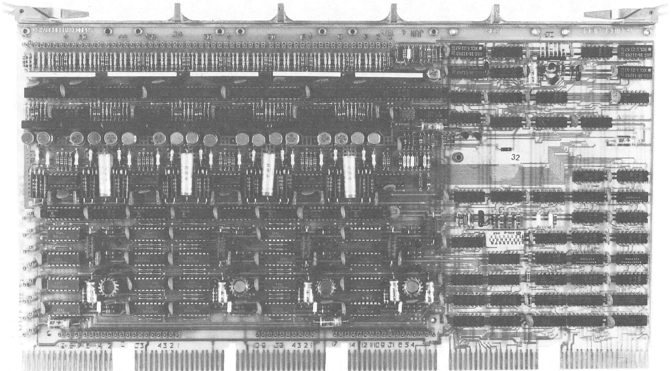
Figure 1-8 MM11-CP Core Memory Module
