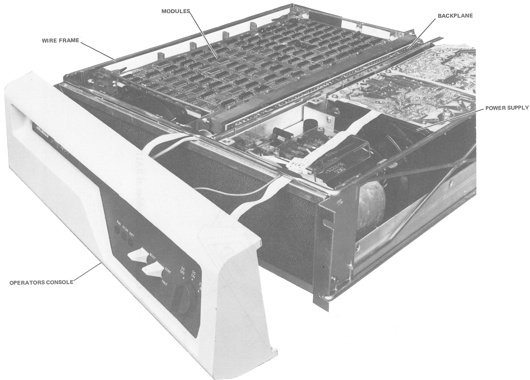
Figure 5-7 Computer Subassemblies of BA11-L Mounting Box
