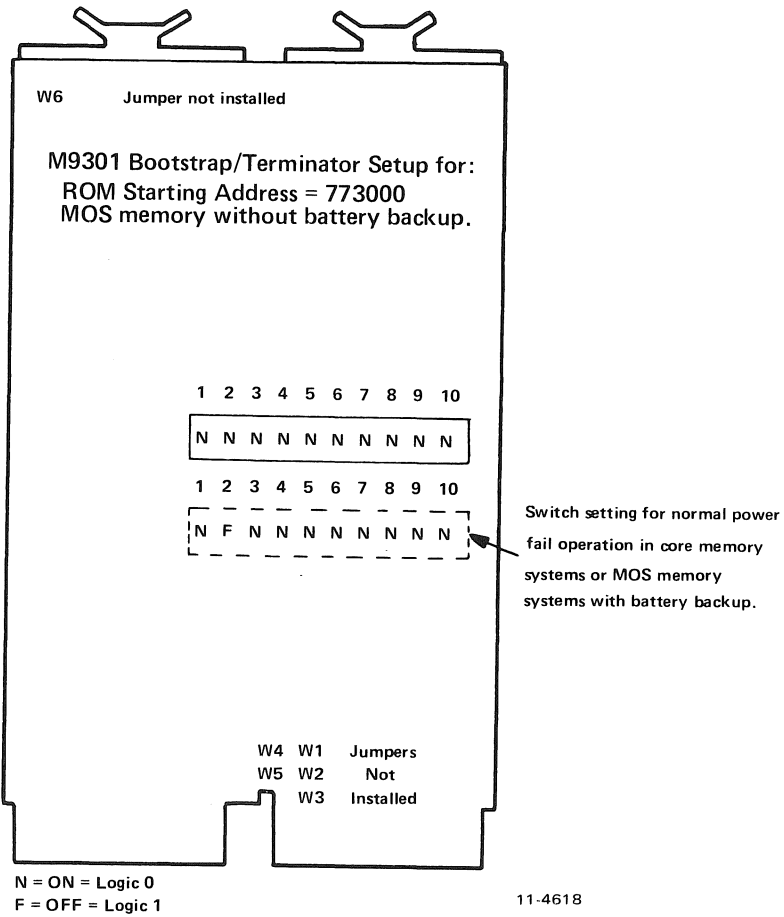
Figure 5-10 Typical Jumper Placement and Switch Settings of Modules (Sheet 2 of 7)
