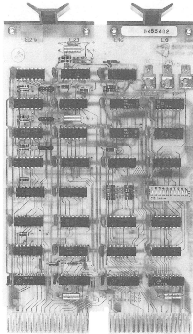
Figure 1-5 M9301 Bootstrap/Terminator Module
