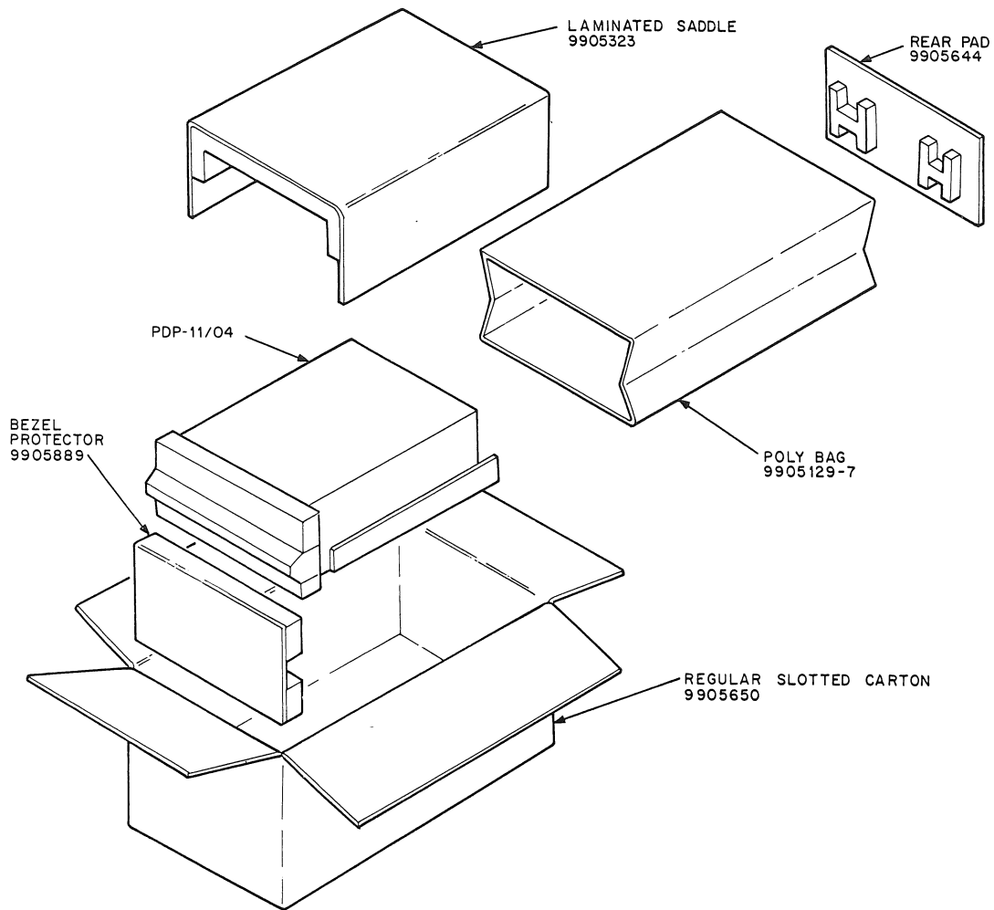
Figure 5-3 Packaging of PDP-11/04 [26.3-cm (10-1/2-inch Box)]
