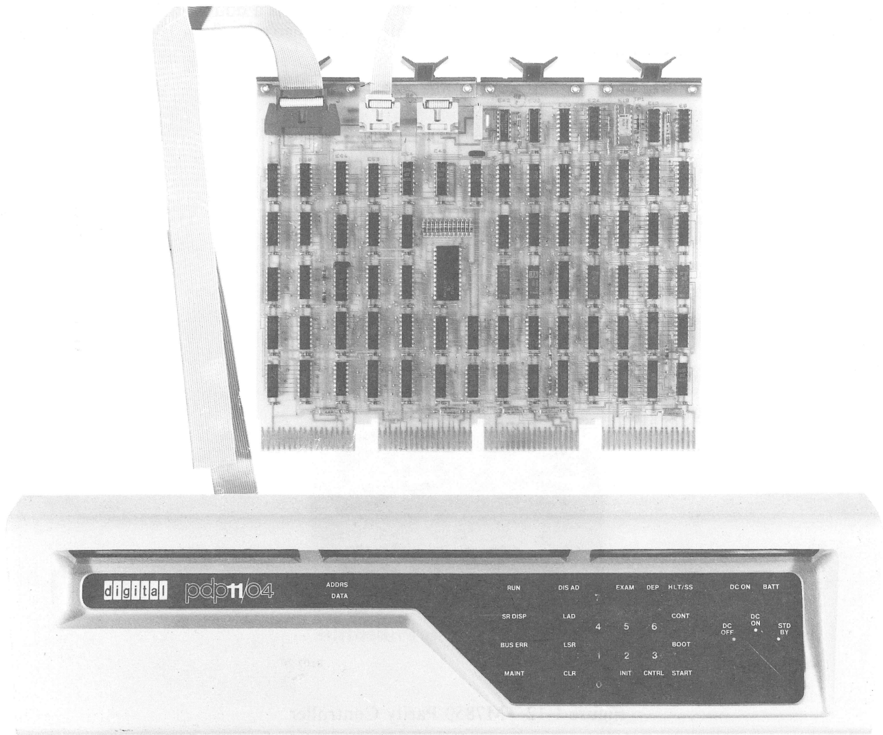
Figure 1-11 KY11-LB Console and Interface Module
