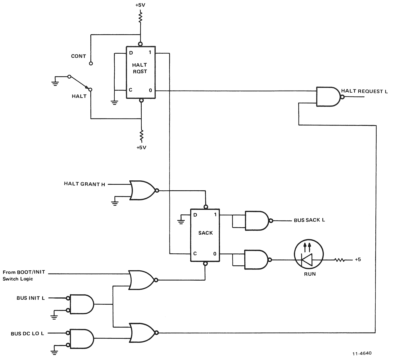
Figure 3-4 HALT/CONT Switch Logic
