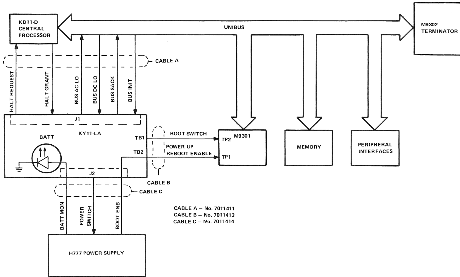
Figure 3-1 PDP-11/04 System Interconnections (BA11-L Mounting Box)
