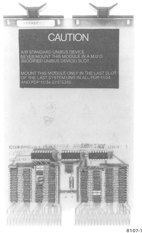
Figure 1-6 M9302 Terminator Module
