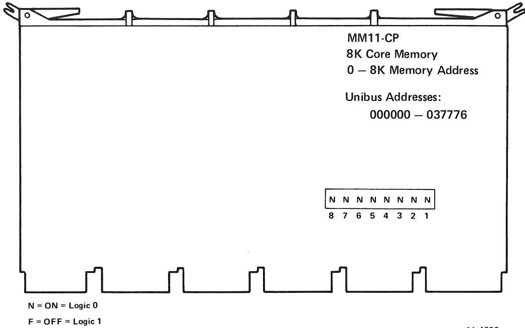
Figure 5-10 Typical Jumper Placement and Switch Settings of Modules (Sheet 6 of 7)
