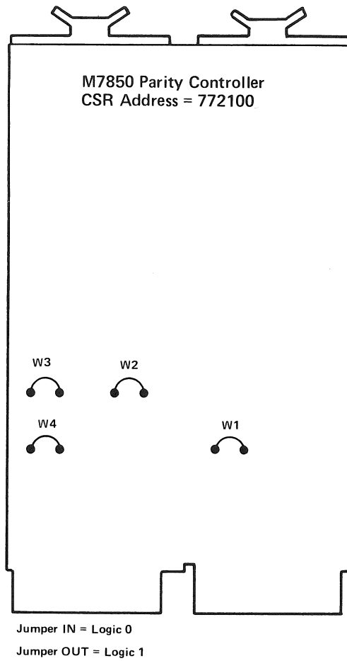
Figure 5-10 Typical Jumper Placement and Switch Settings of Modules (Sheet 1 of 7)
