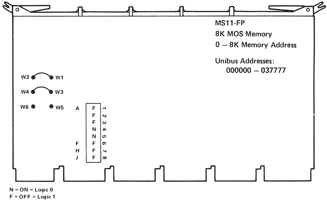
Figure 5-10 Typical Jumper Placement and Switch Settings of Modules (Sheet 4 of 7)
