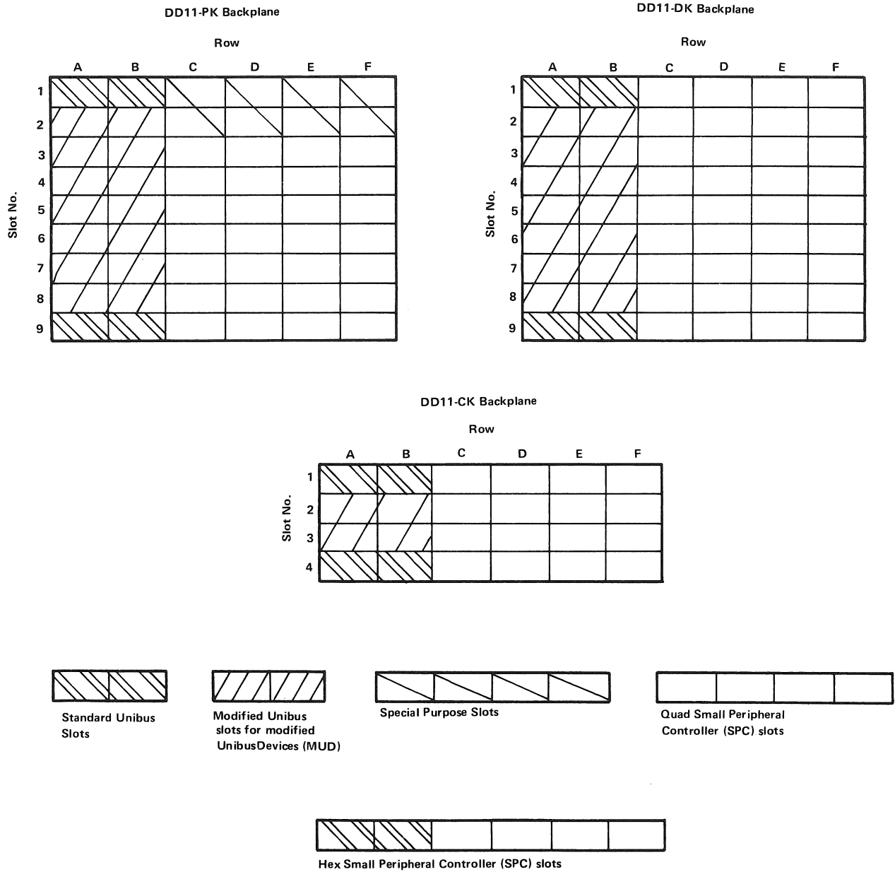
Figure 4-1 PDP-11/04 Backplanes
