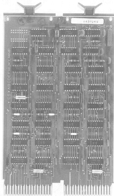
Figure 1-12 M7850 Parity Controller
