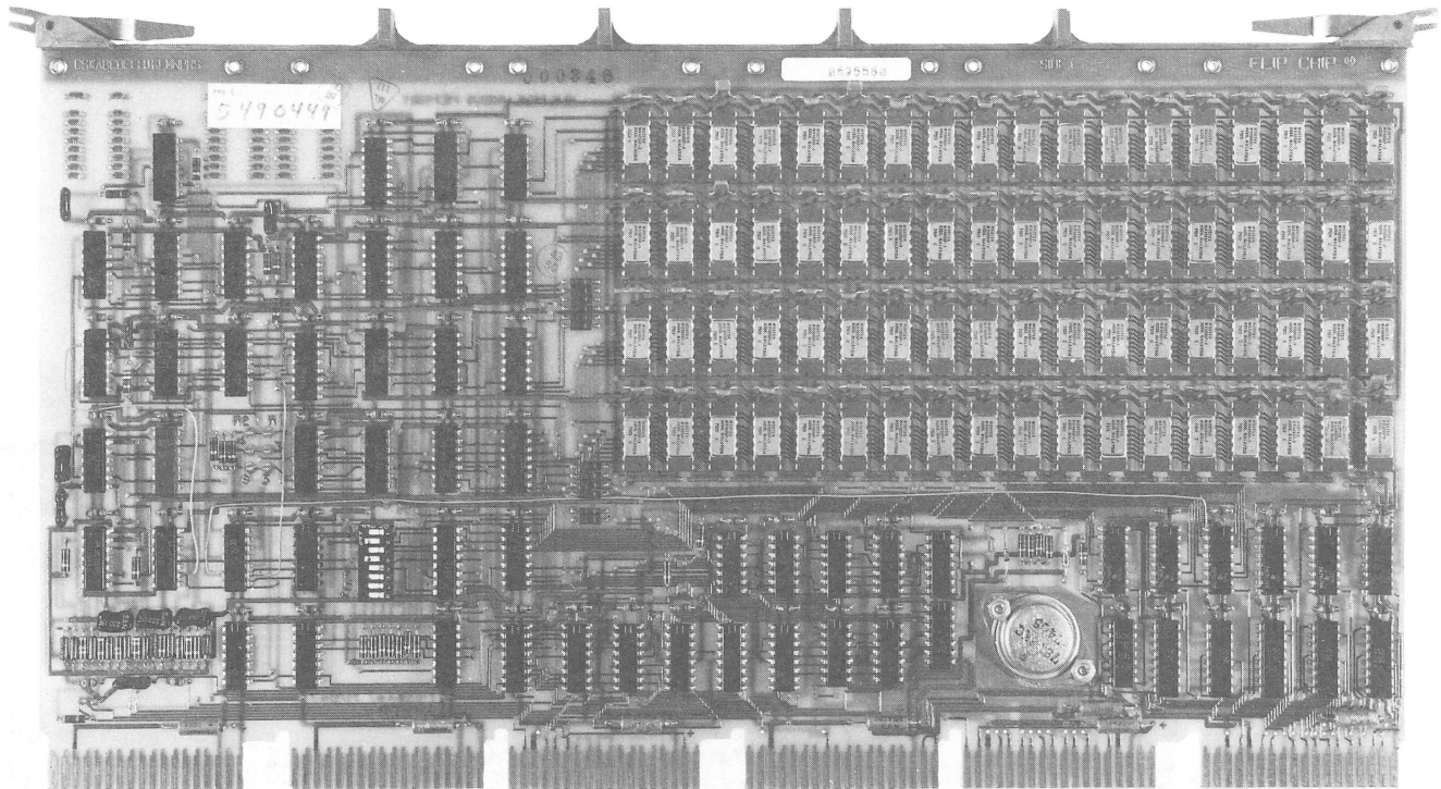
Figure 1-7 MS11-JP MOS Memory Module
