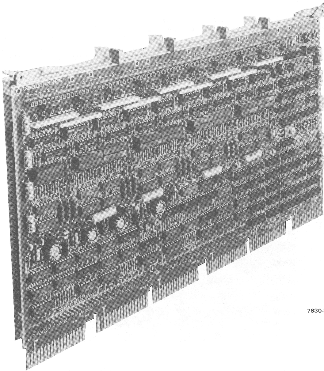
Figure 1-9 MM11-DP Core Memory Module
