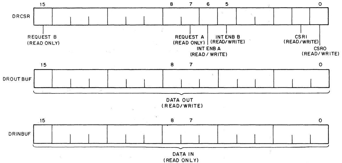
Figure 5-6 DRV11 Word Formats
